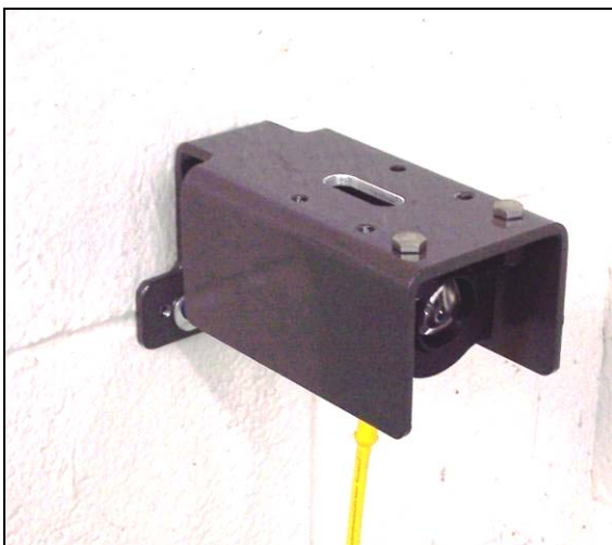
Pic #8: Photo-Eye Guard Wall Mounted
